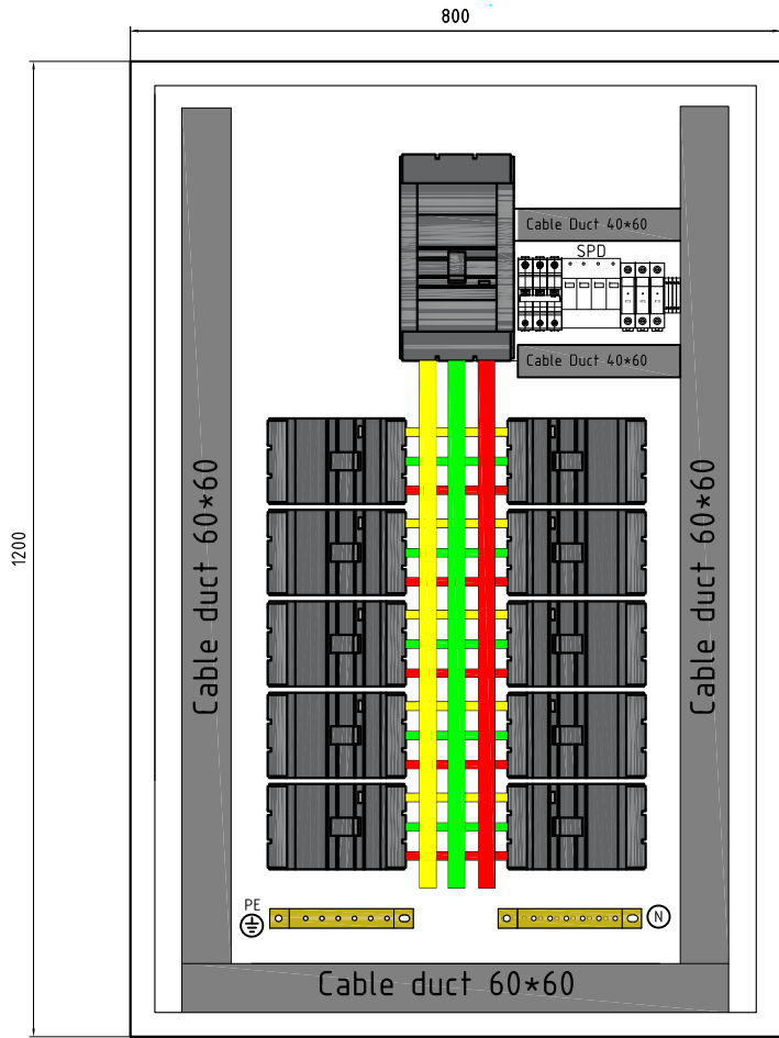
INSIDE VIEW
